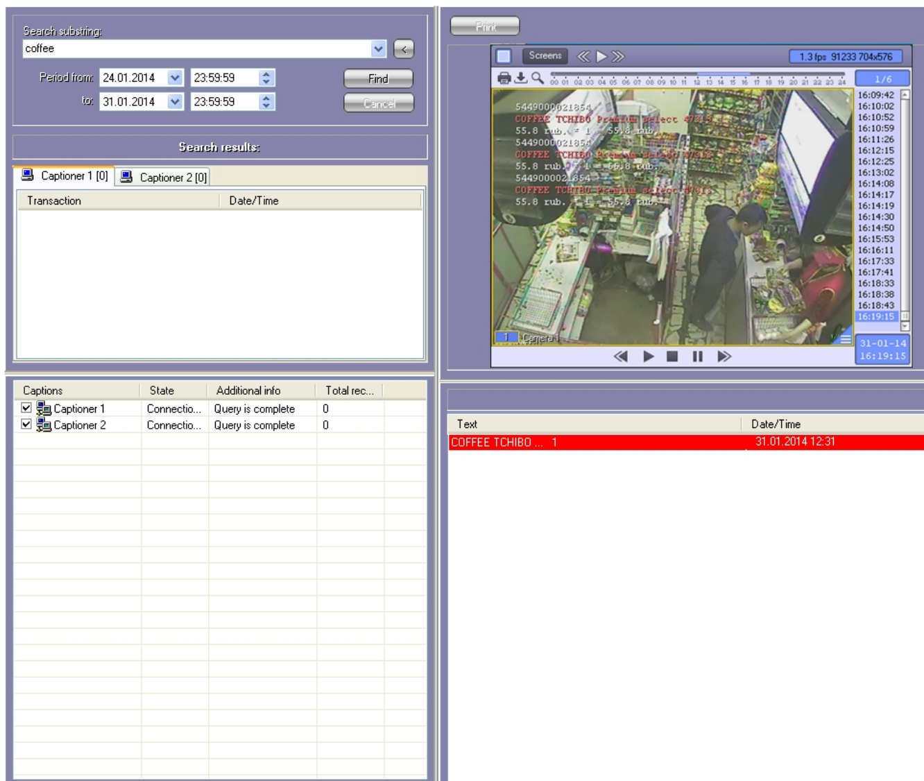
Changing the window layout (initial layout)
