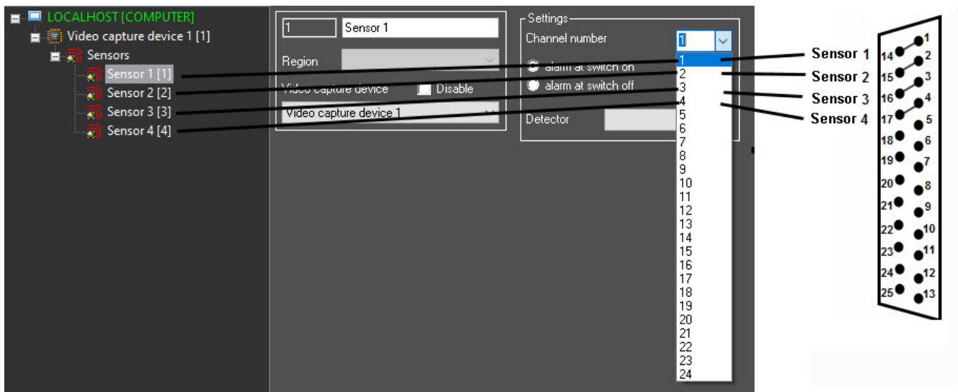
Channels of the second 4/4 Sensor-Relay card (low profile) are numbered 1-4.
