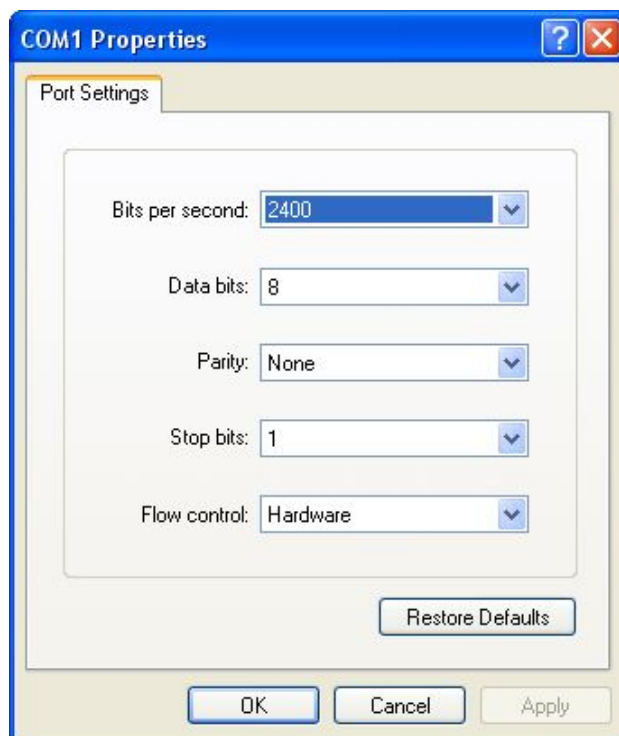
Figure 6.3.8.3-7 COM connection settings
