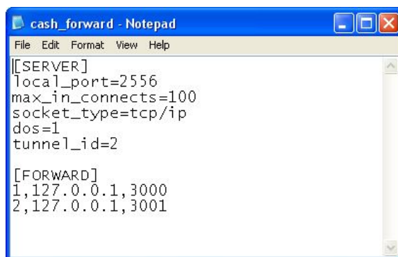
Figure 6.3.8.3-1 The cash_forward.ini file
