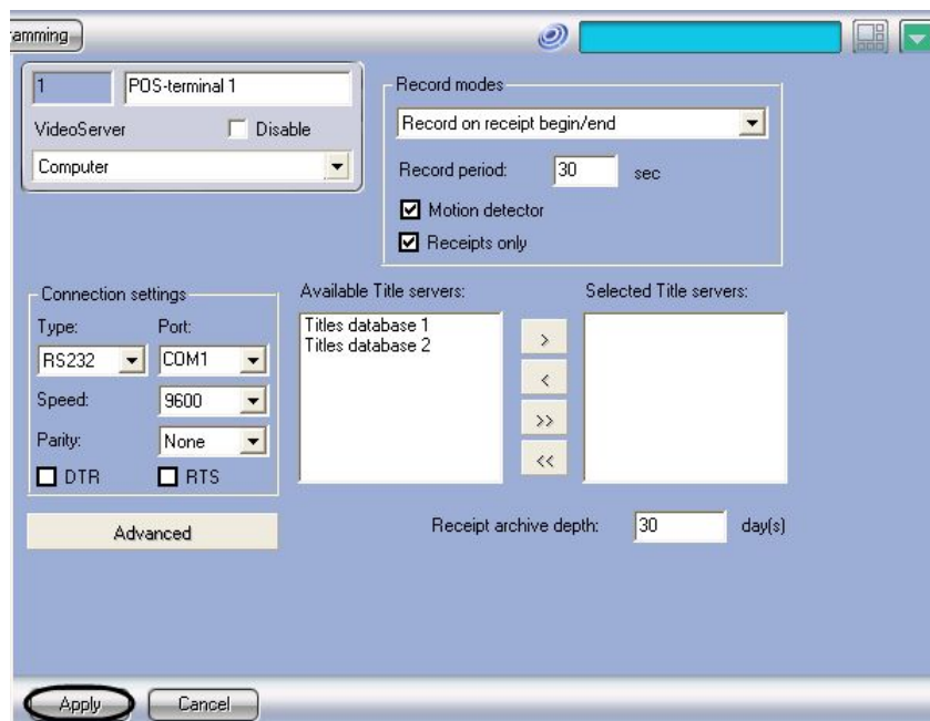
Figure 6.3.8.1-4 Saving the changes
