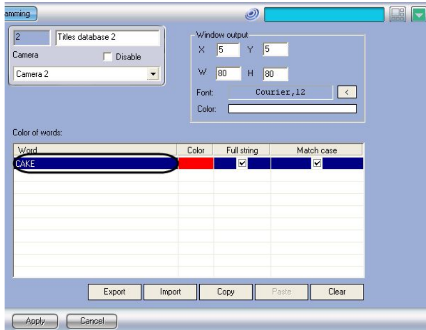
Figure 6.3.8.1-3 Adding the new rule to the Word highlighting table
