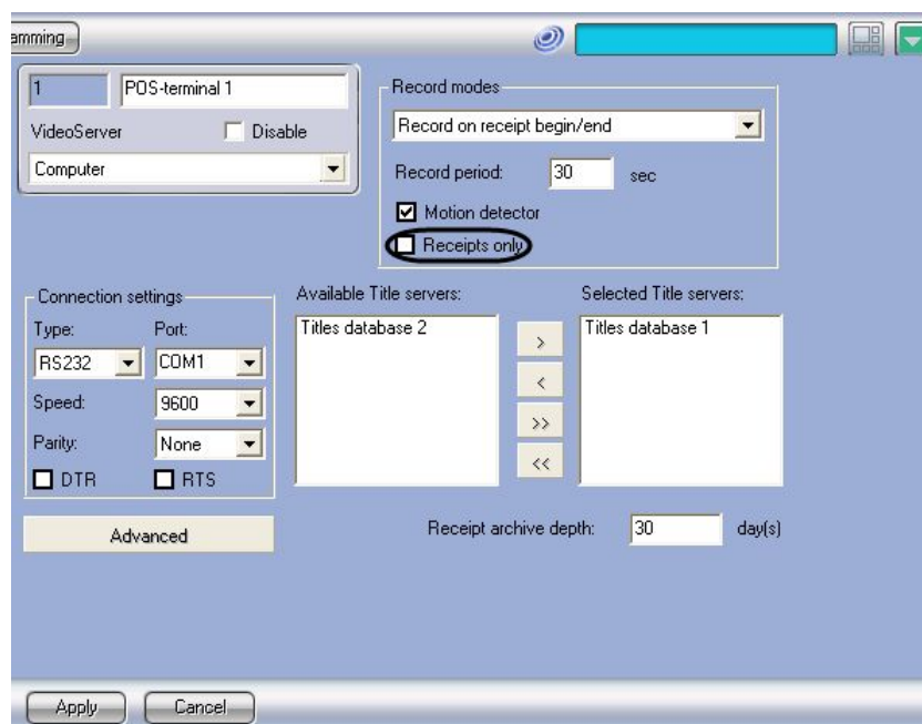
Figure 6.3.8.1-3 The Receipts only option
