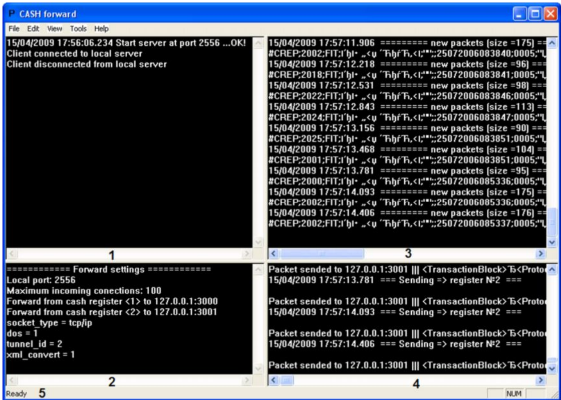
Figure 6.3.8.3-1 The CASH forward window
