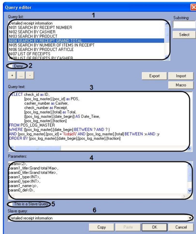
Figure 6.3.8.3-10 Query text display
