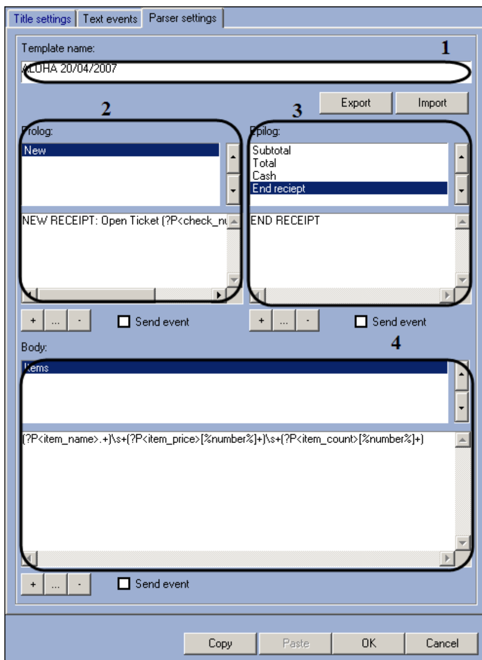
Figure 6.3.8.3-4 Settings group on the Parser settings panel
