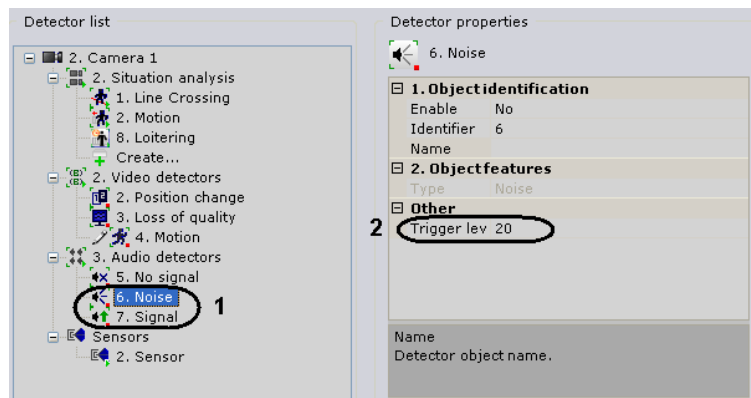
Fig. 6.4—18 Configuration of the Signal and Noise Detectors
