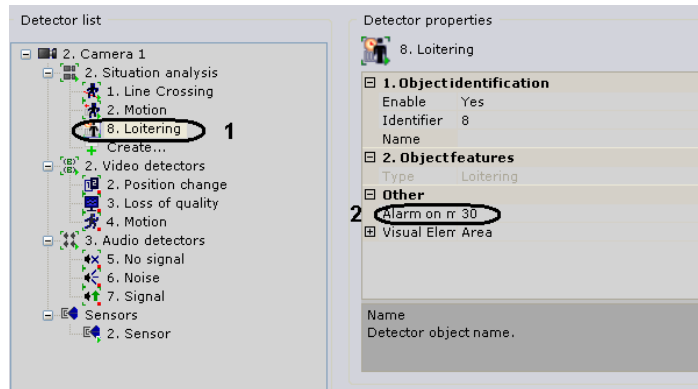
Fig. 6.4—10 Configuring the loitering detector
