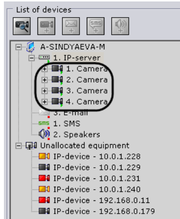
Fig. 6.3—11 An IP server object in the objects tree
