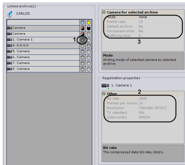
Fig. 6.5—5 Configuring recording from a video camera to an archive
