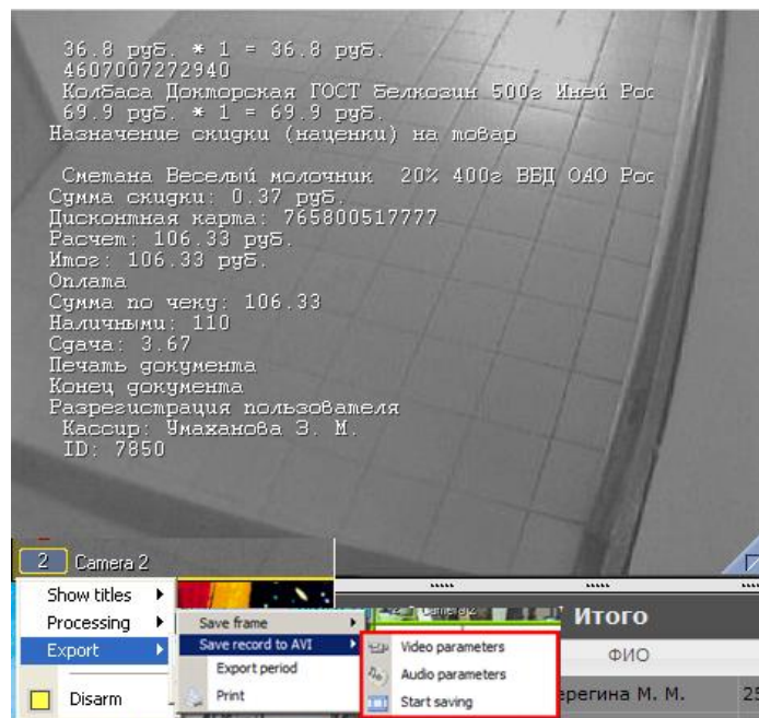
Figure 8.1—14 Video export
