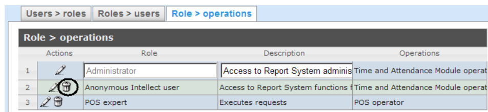
Figure 7.1—3 Role removing
