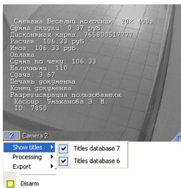
Figure 8.1—15 Show titles
