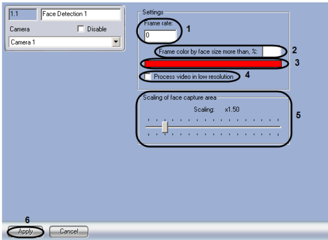
Figure 8.2-2 Face detection setting panel
