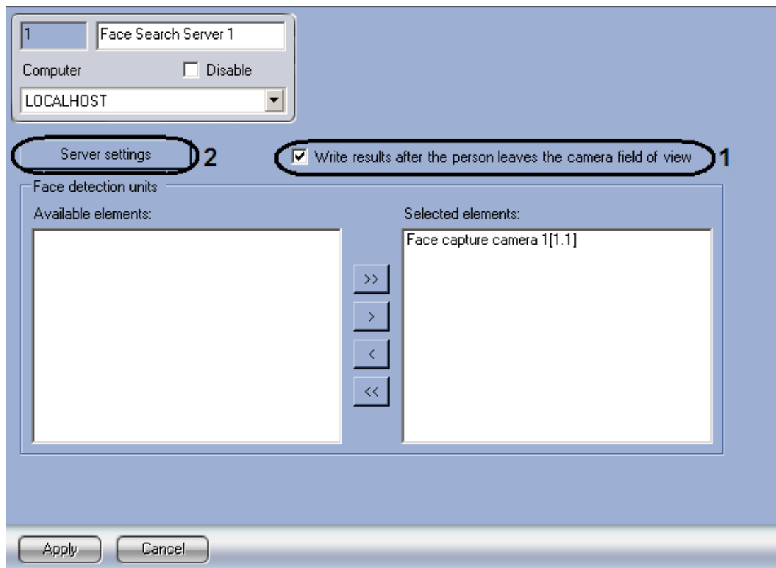
Figure 8.3-2 Face search server object setting panel
